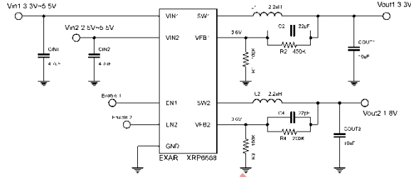
Fig. 22: Typical Application
