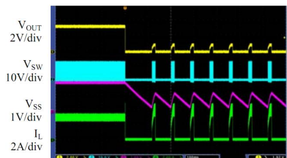
Time 100ms/div Fig. 14: Short-circuit protection I_{OUT}=3A
