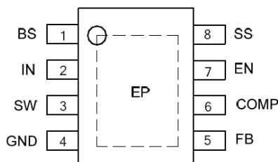
Fig. 3: XRP7675 Pin Assignment (Exposed Pad SOIC-8)
