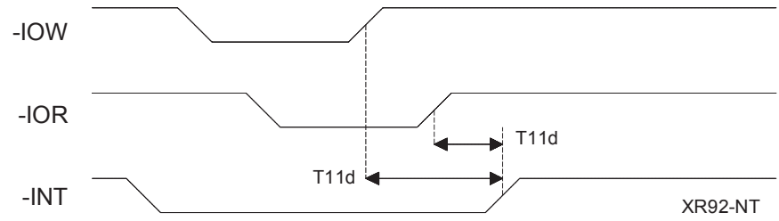
Figure 8: Interrupt Timing
