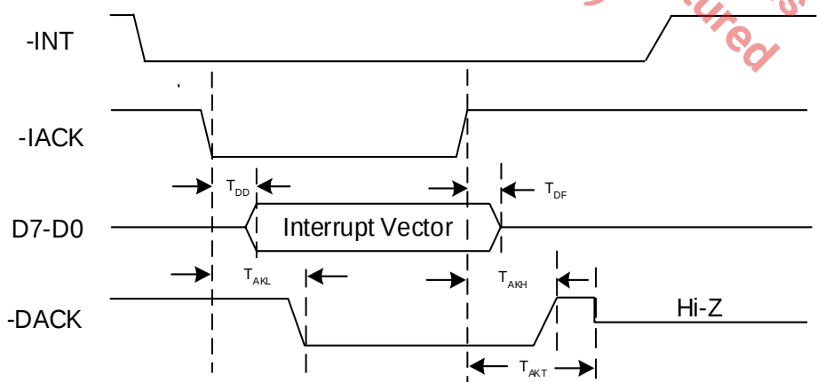
Figure 7: Interrupt Timing
