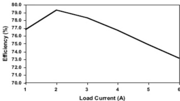
Fig. 7: Efficiency versus Output Current V_{IN}=3.3V , V_{OUT}=0.8V
