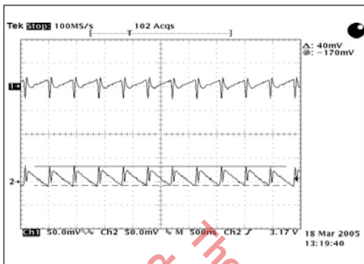
Fig. 10: Ripple 1x Torch 150mA, Ch1=V IN , Ch2=V OUT V IN =4.2V, C IN =4.7μF, C FC =0.47μF, C OUT =2.2μF
